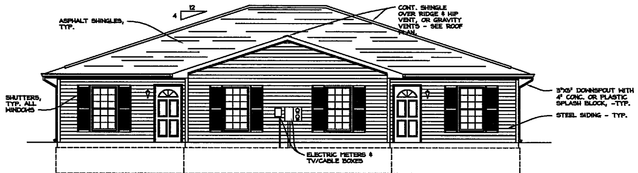
③ REAR ELEVATION SCALE: 3/16" = 1'-0"
