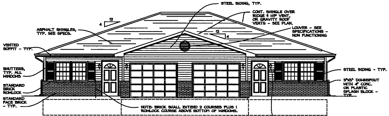
① FRONT ELEVATION SCALE: 3/16" = 1'-0"
