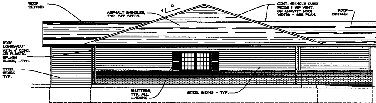
② SIDE ELEVATION (SAME ON OTHER SIDE) SCALE: 3/16" = 1'-0"
