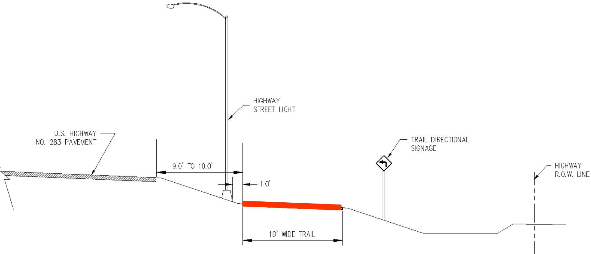
TYPICAL TRAIL SECTION NO SCALE
