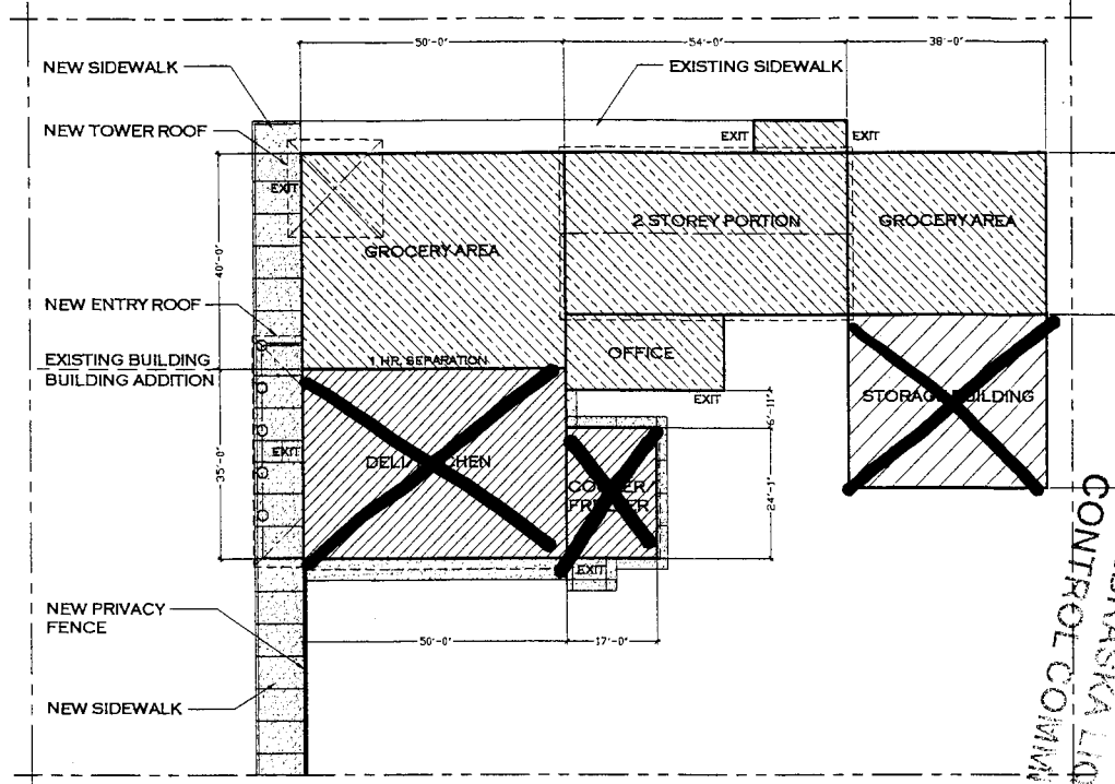
1 SITE PLAN - EXISTING AND ADDITIONS SCALE: 1/8" = 1'-0"
